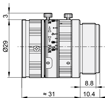
Basler Lens with f = 4 mm, 6 mm, 8 mm
