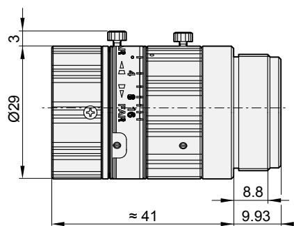
Basler Lens with f = 12 mm, 16 mm, 25 mm
