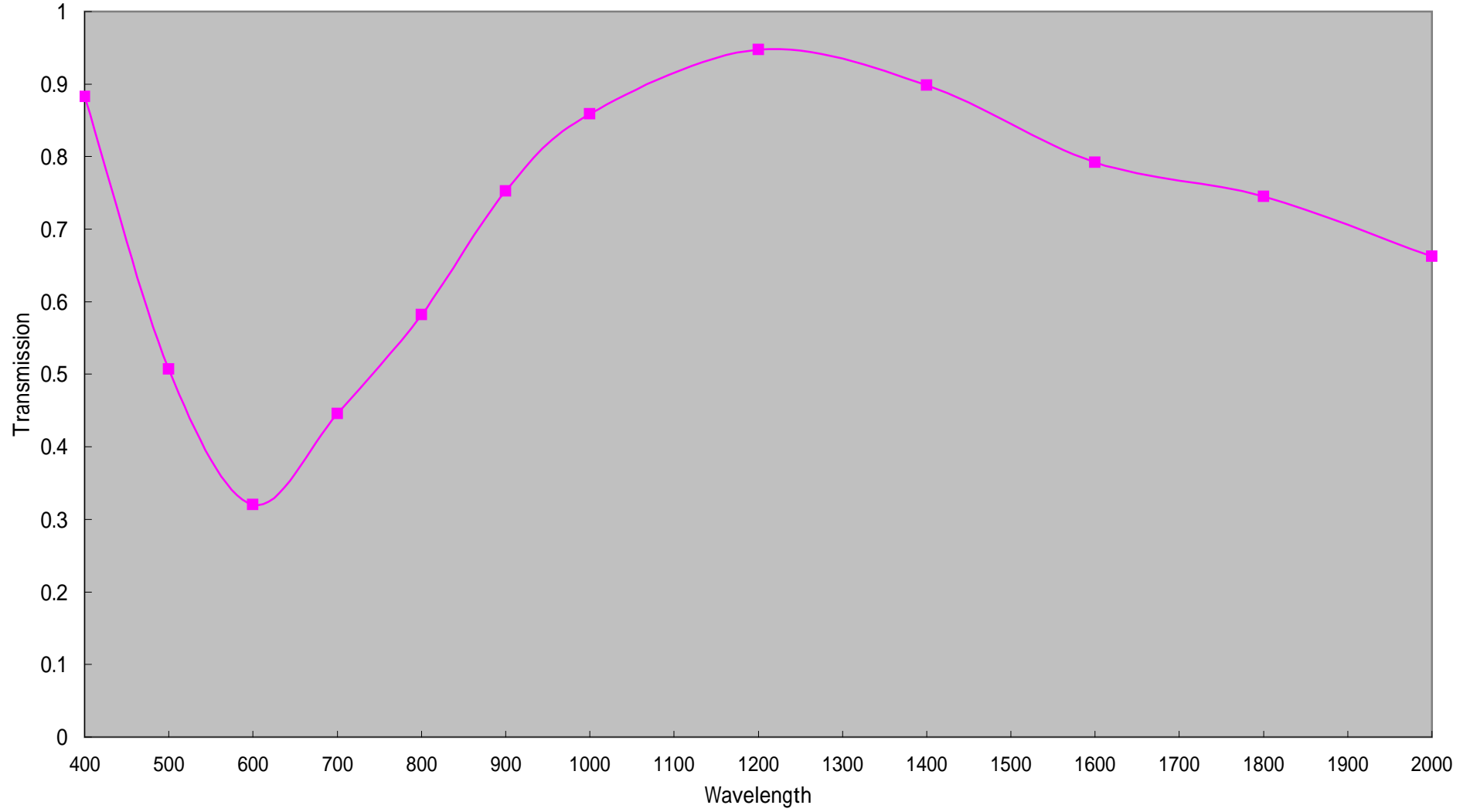
LM25HC-SW Transmission
