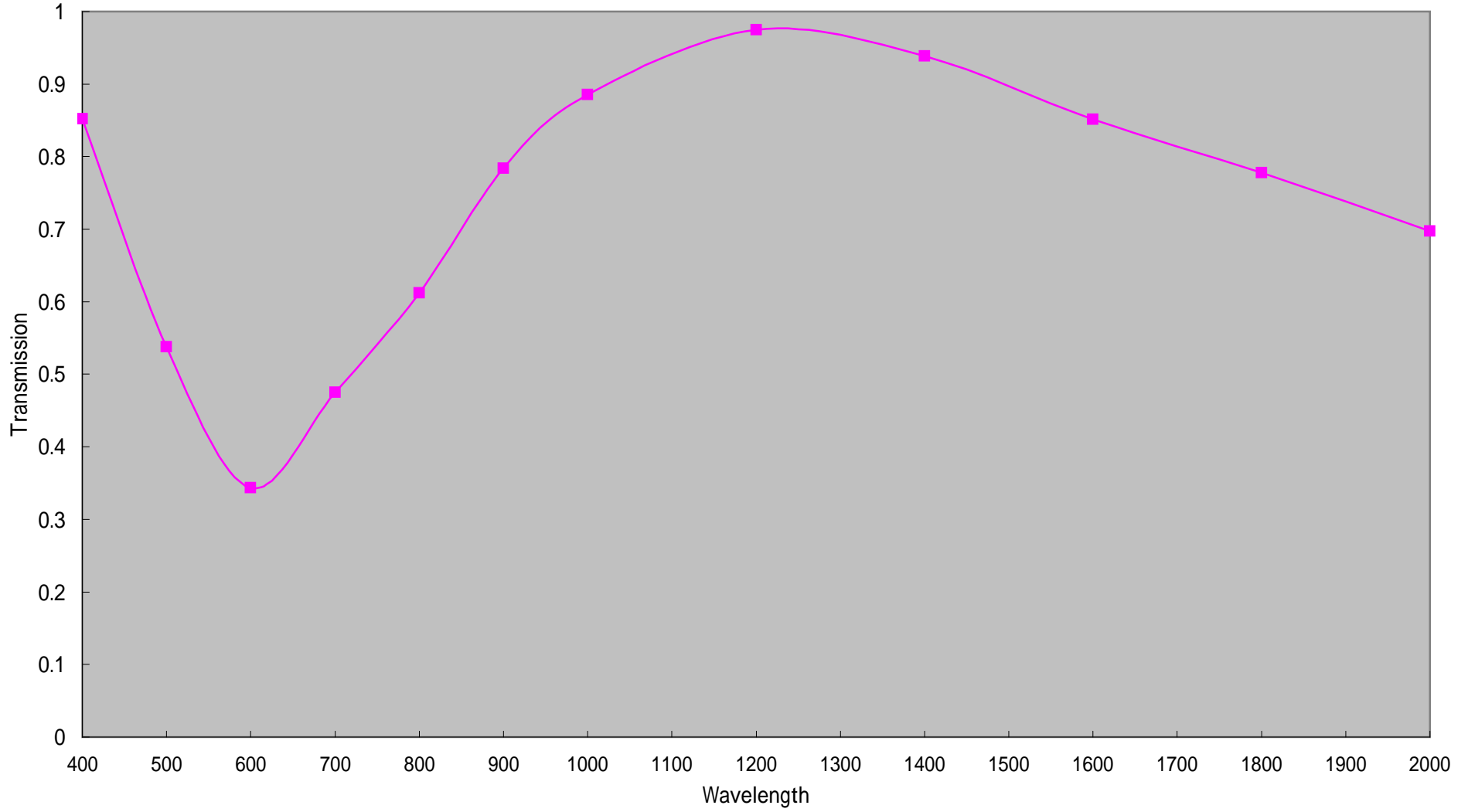
LM35HC-SW Transmission
