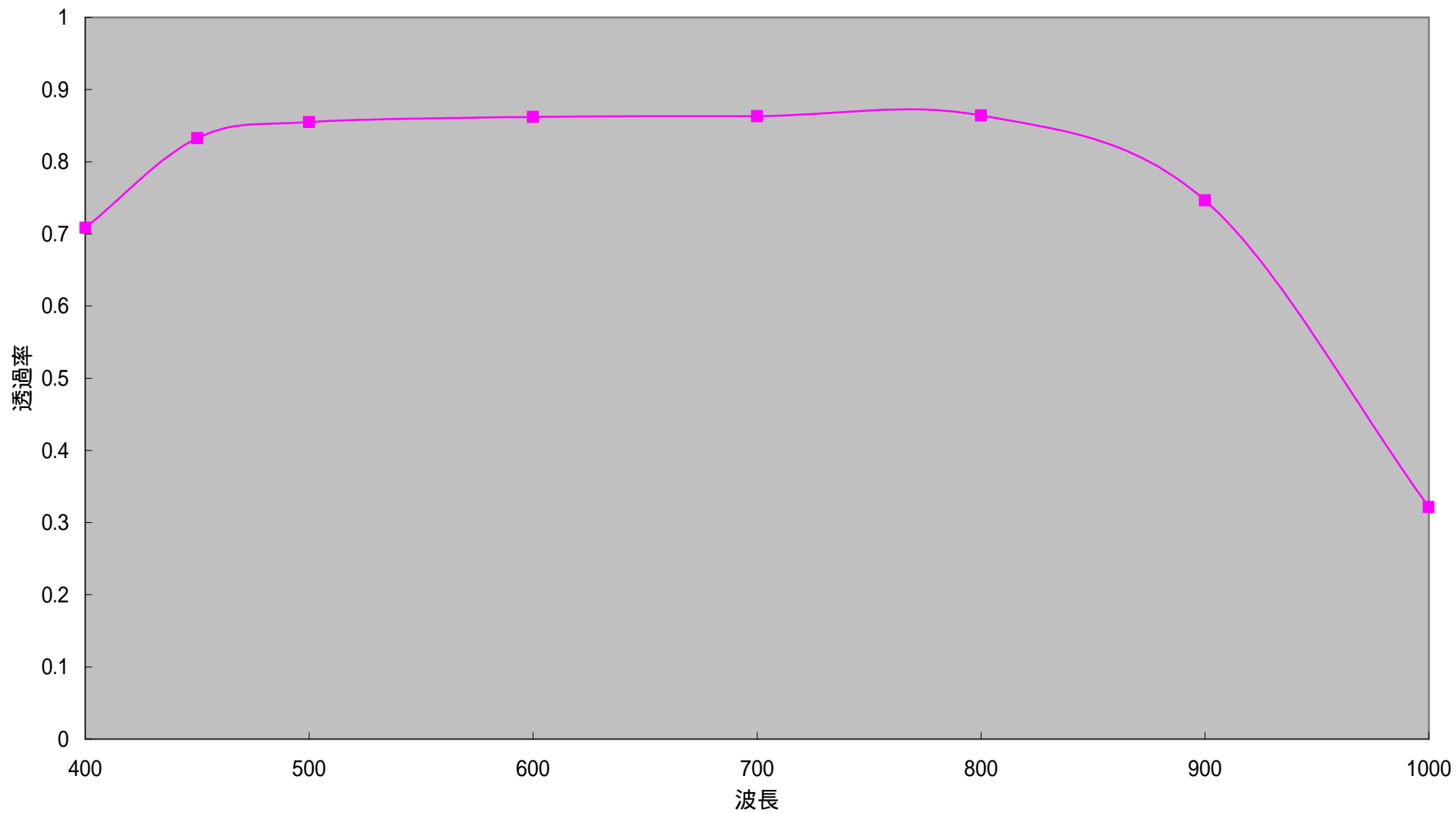
LM25JC10M 透過率
