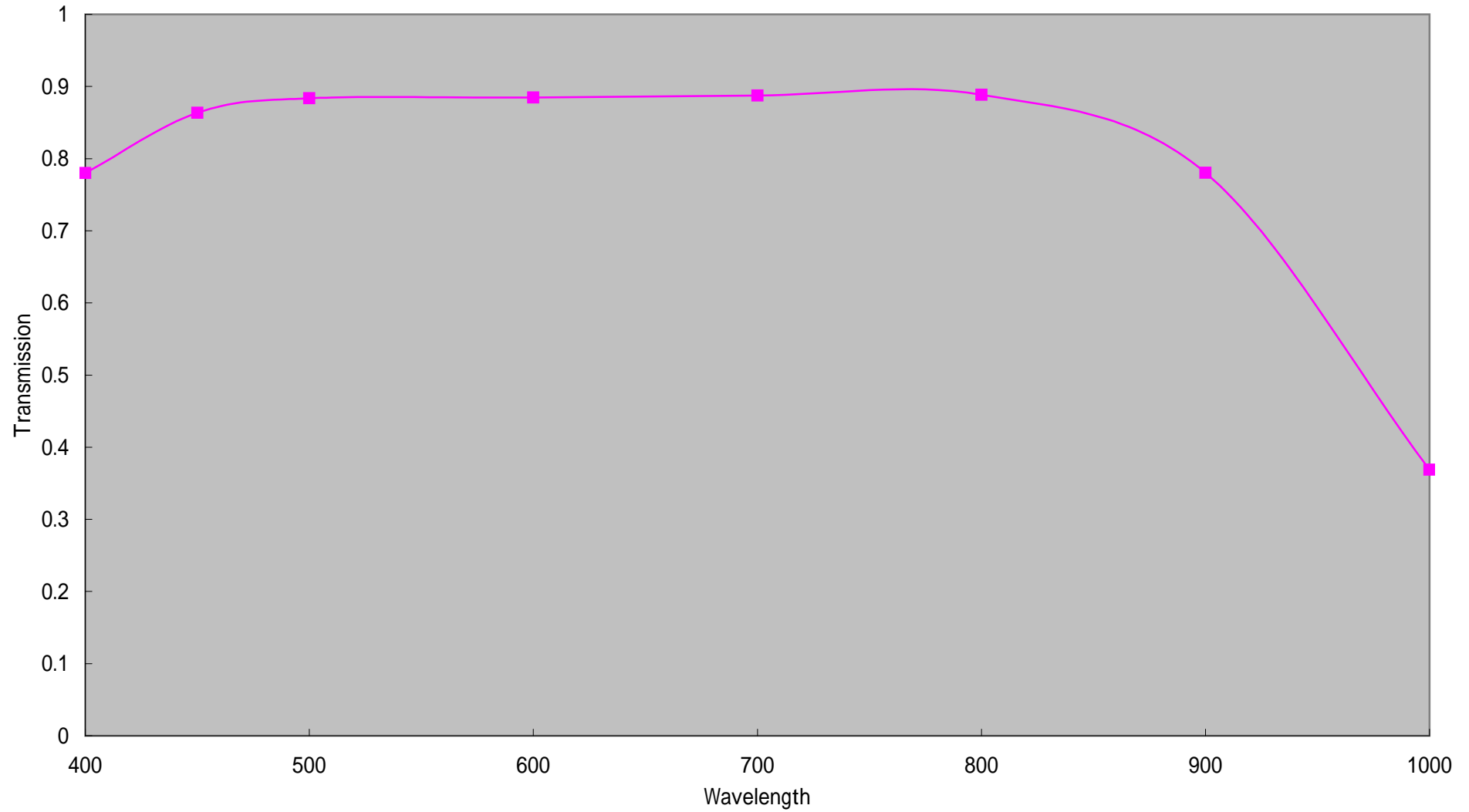
LM35JC10M Transmission
