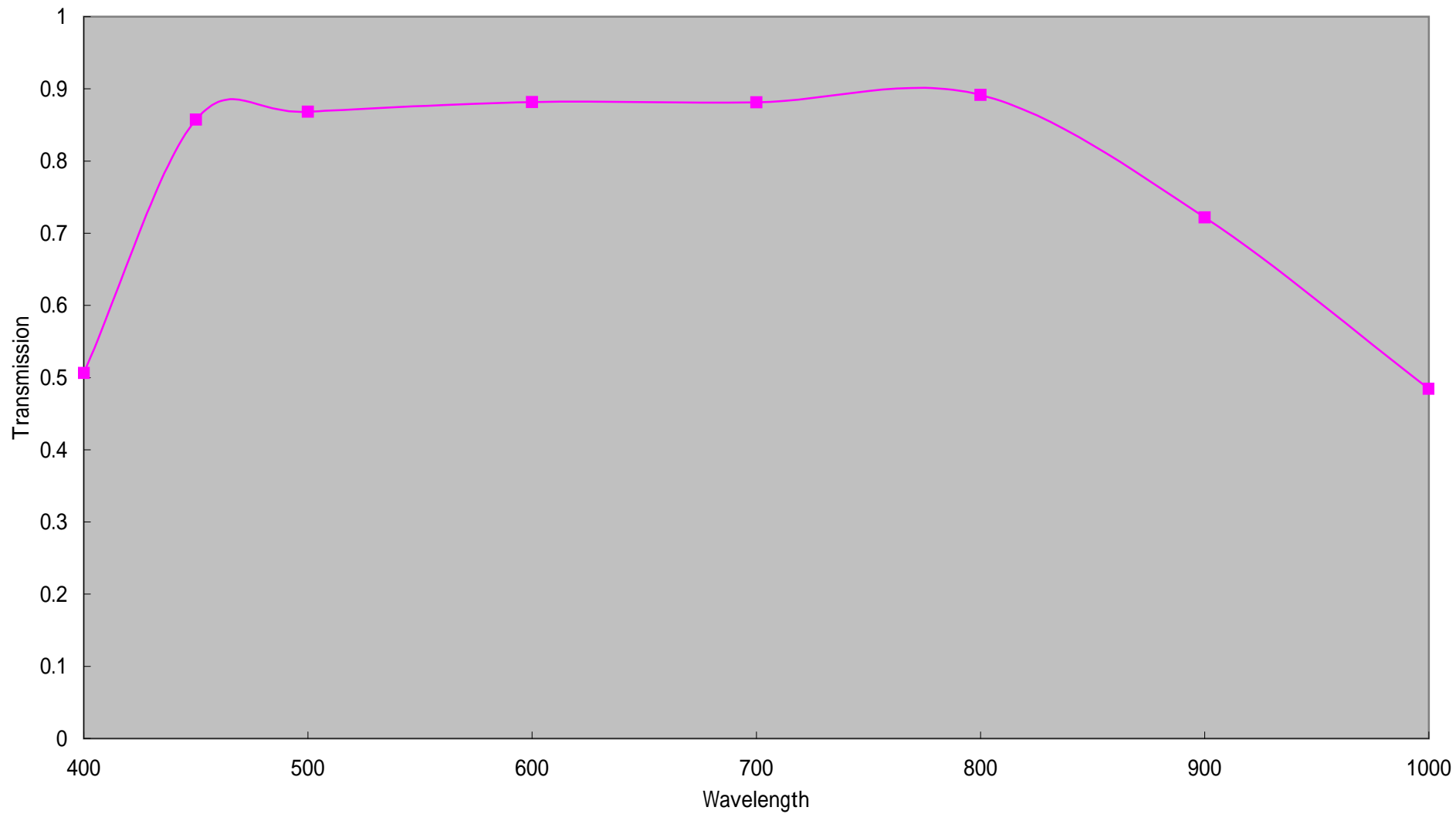
LM35LF (1036) Transmission
