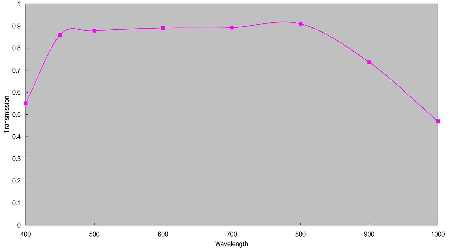
LM50LF (1037) Transmission
