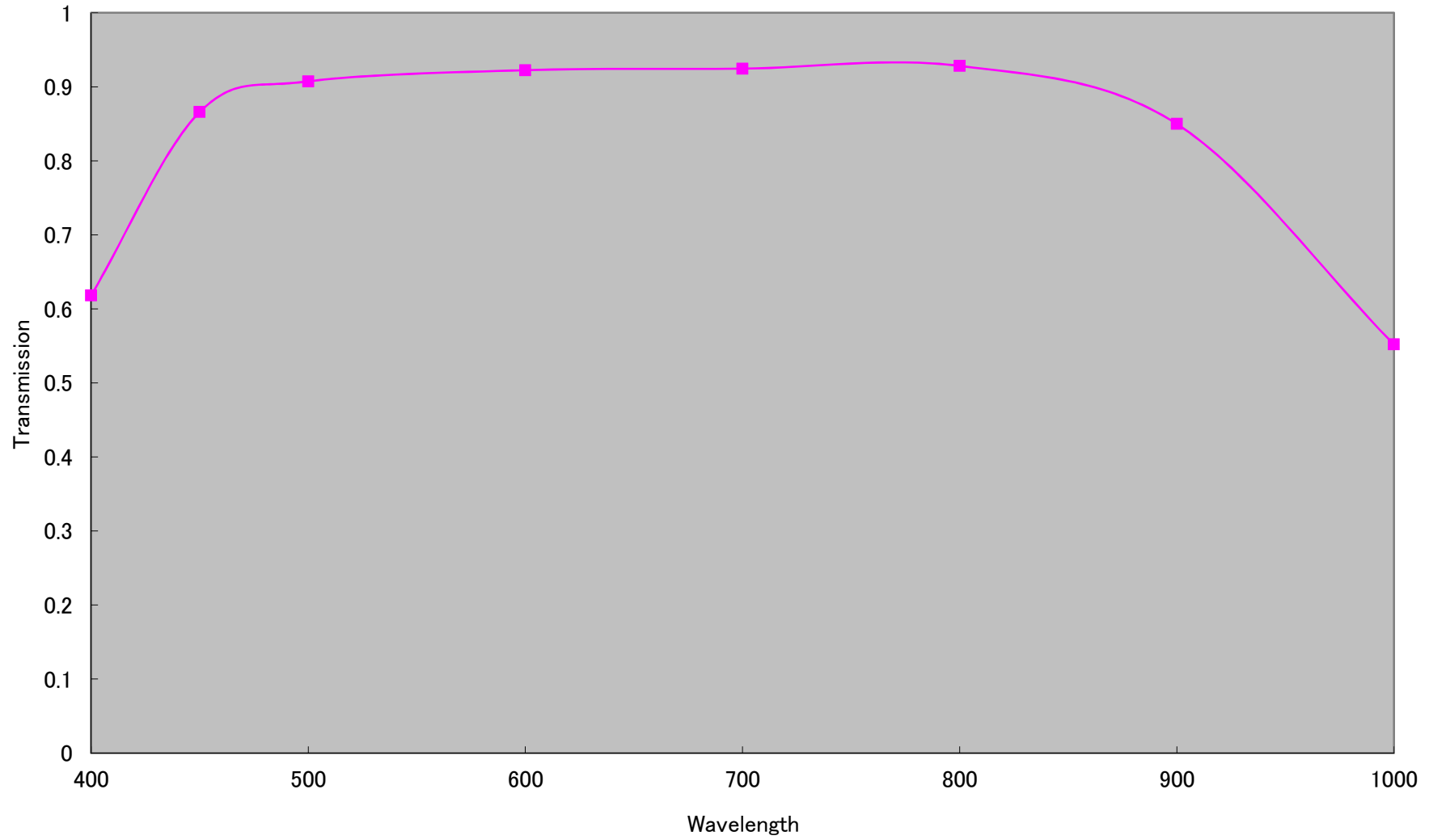
LM50SC Transmission
