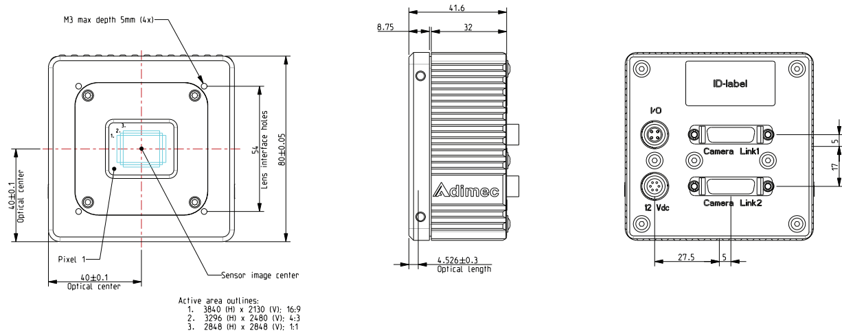
Figure 5. Mechanical Outline
