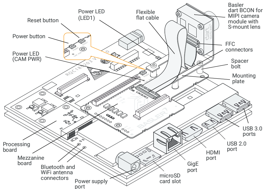
Fig. 1: daA2500-60mc-SD820-DB8 – Installed Hardware Components
