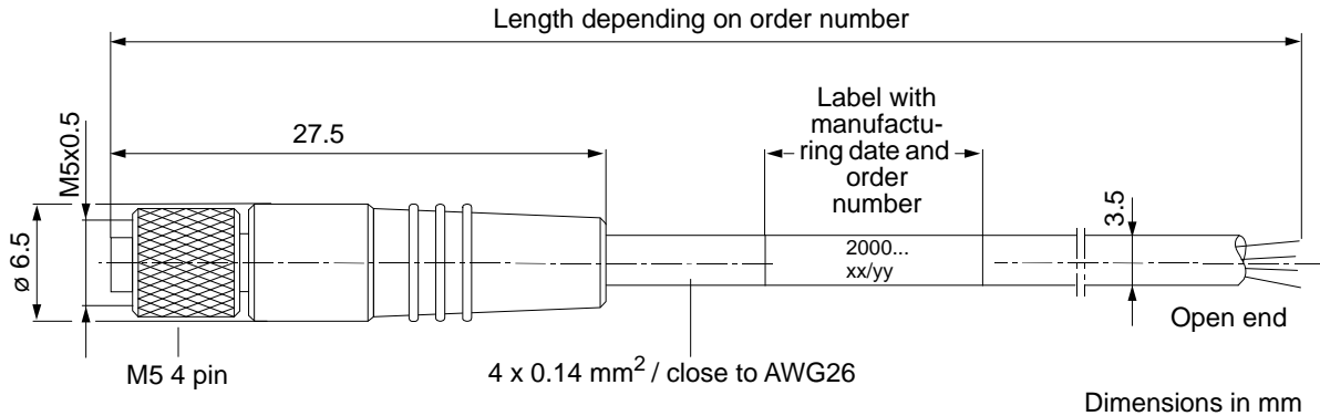
Fig. 1: Cable Overview
