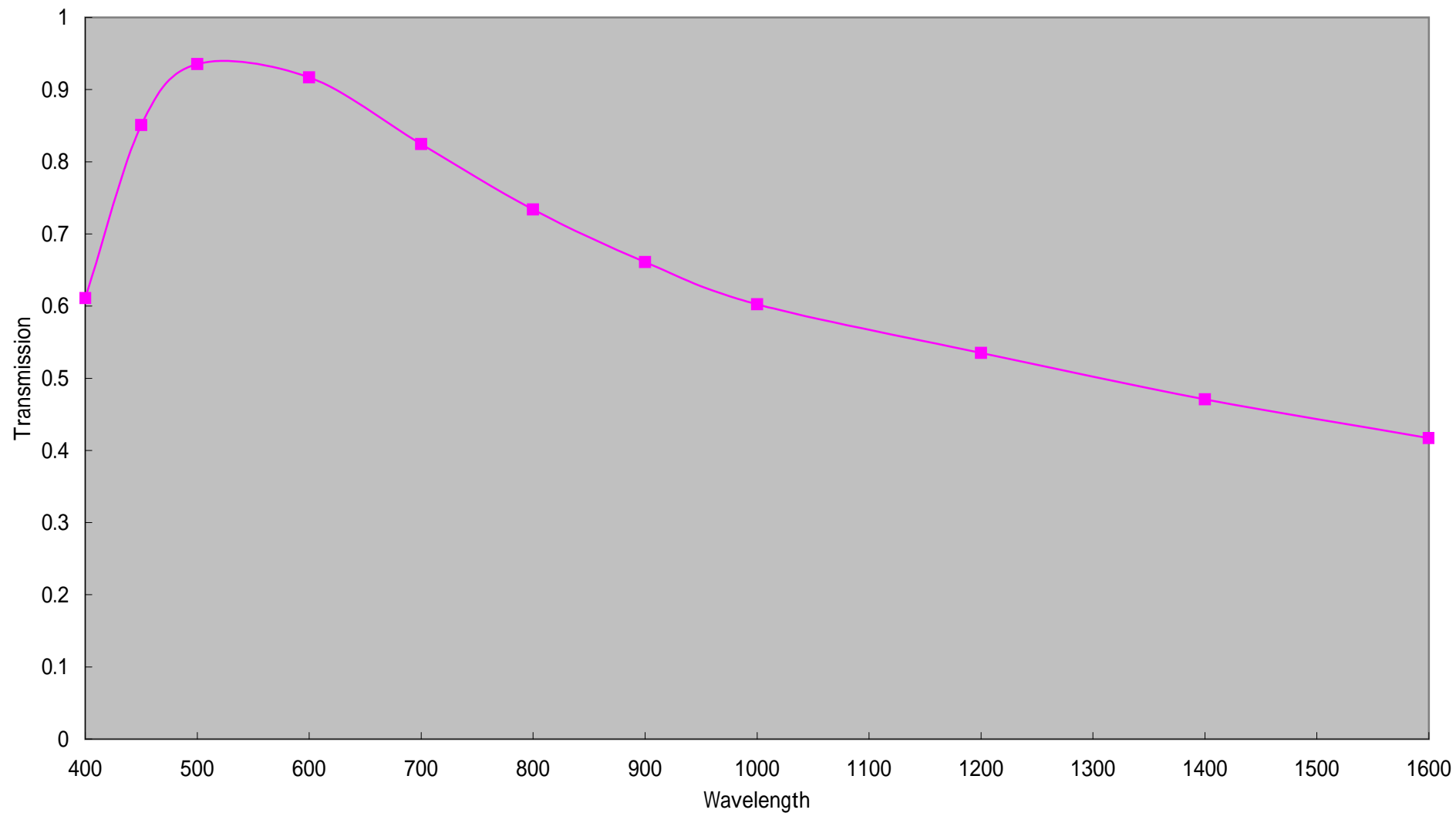
LM35JCM Transmission
