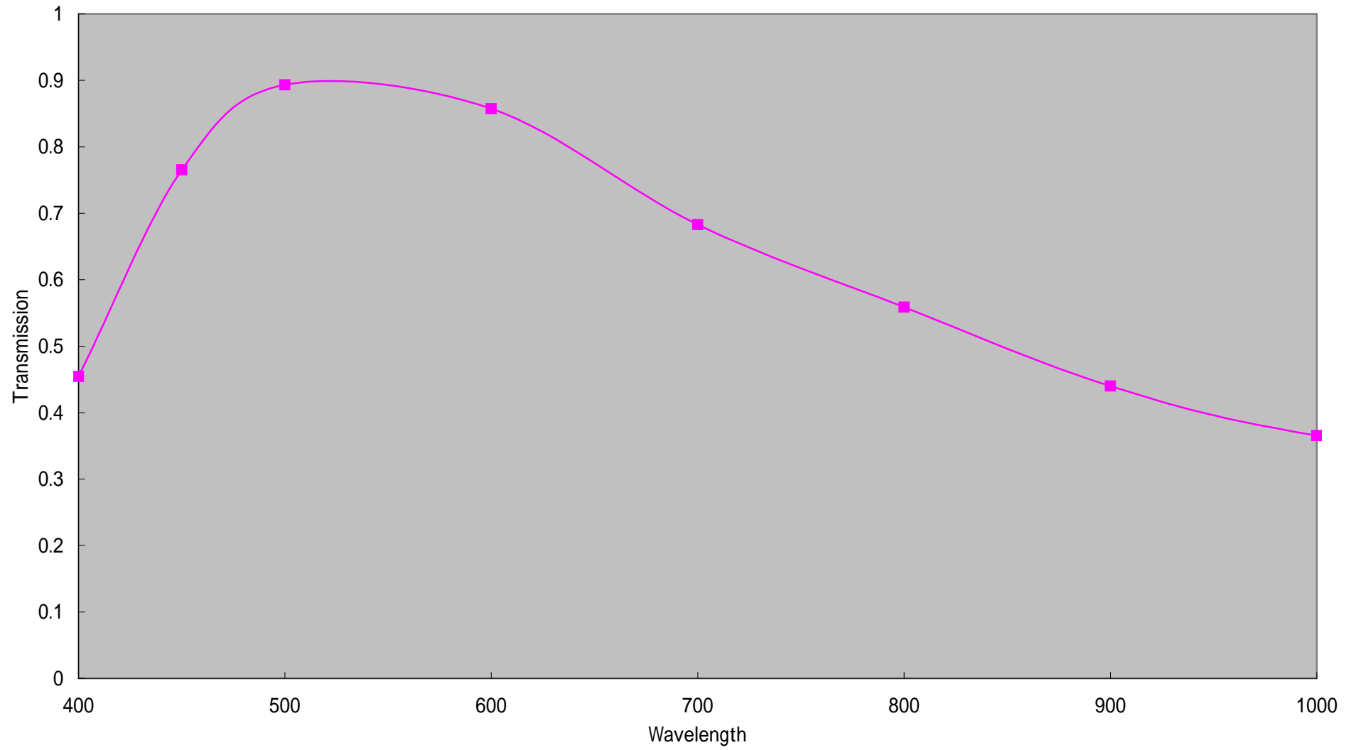
LM6HC (1059) Transmission
