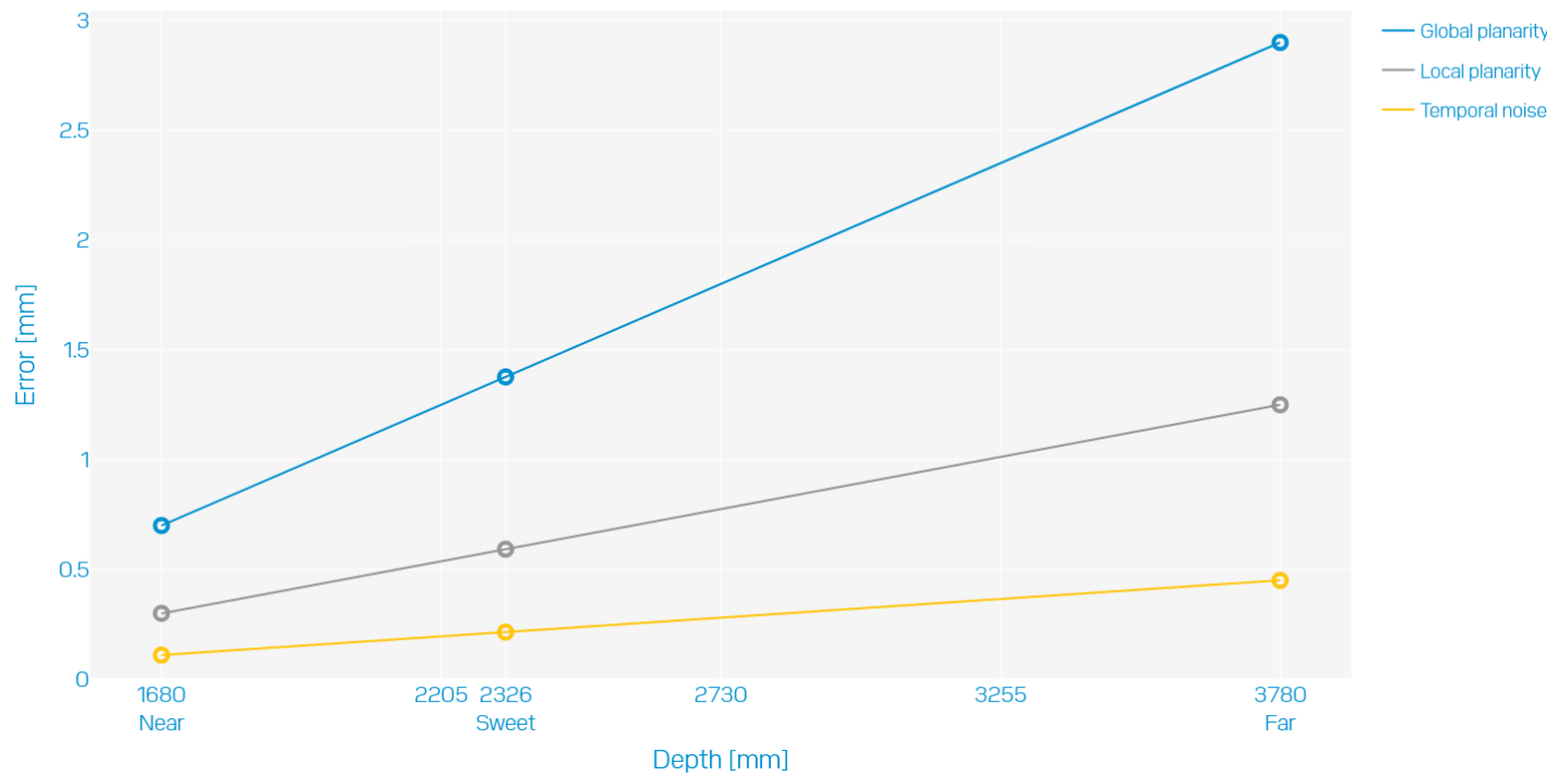
Planarity and temporal noise PhoXi 3D Scanner XL Gen3 (Blue)
